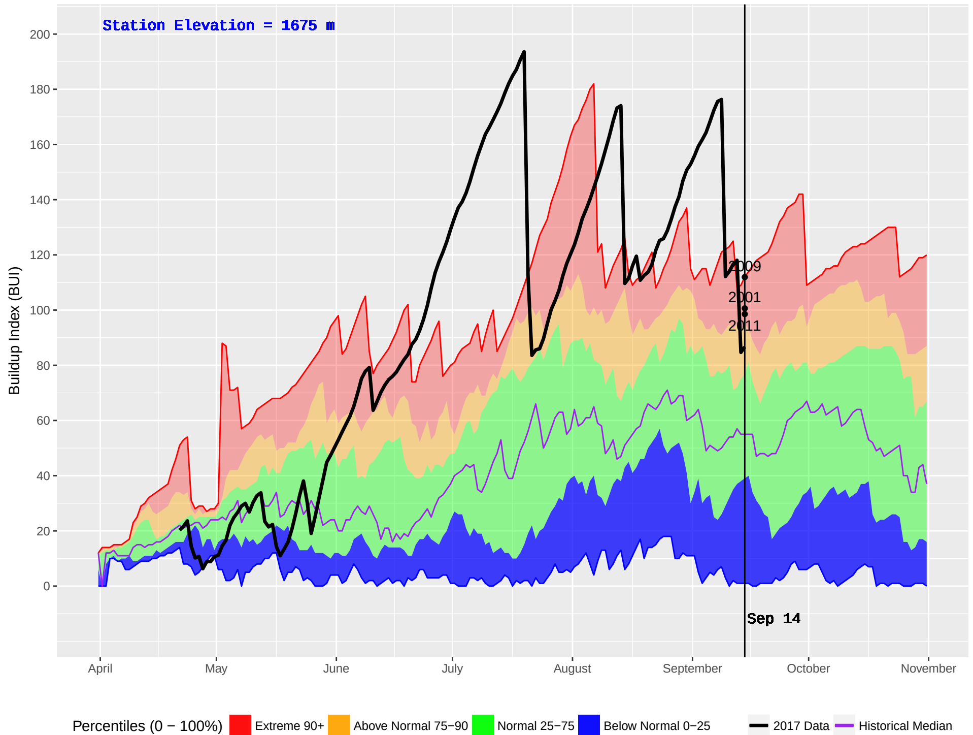
GASPARD (222) : Historical (1992–2016) and Current (2017) Noon Buildup Index (BUI)
