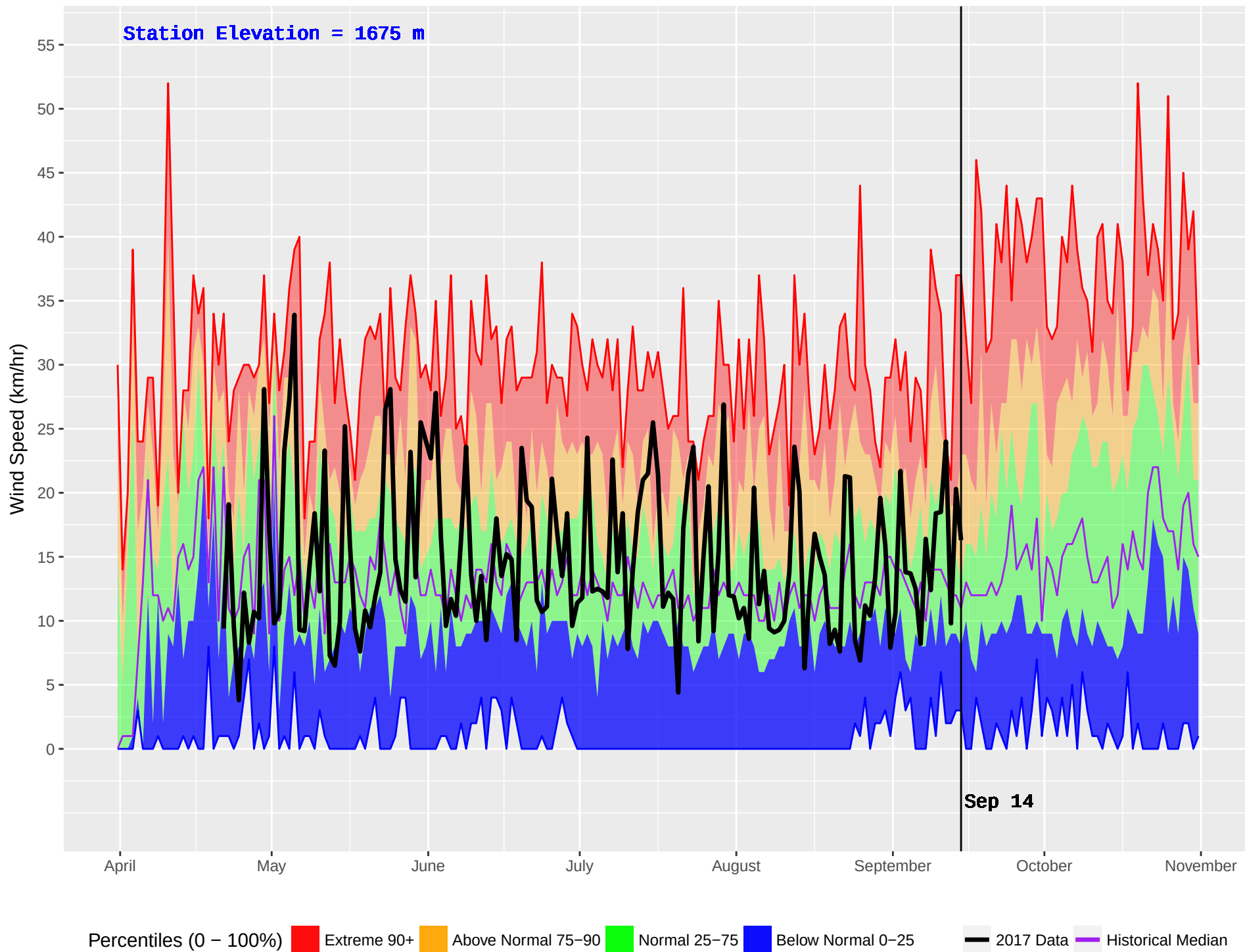
GASPARD (222) : Historical (1992–2016) and Current (2017) Noon Wind Speed
