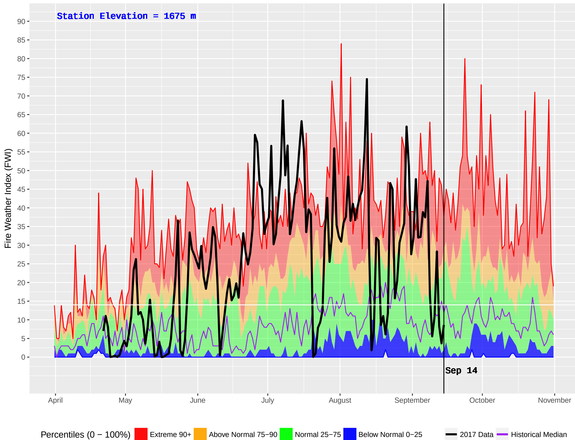
GASPARD (222) : Historical (1992–2016) and Current (2017) Noon Fire Weather Index (FWI)
